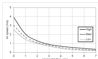
MMK-UP0071HP-E
