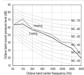
MMY-MUP1001HT8(J)P
