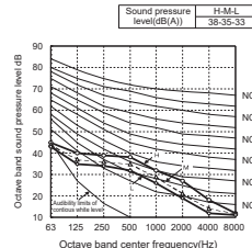
MMU-UP0241WH-E, MMU-UP0271WH-E
