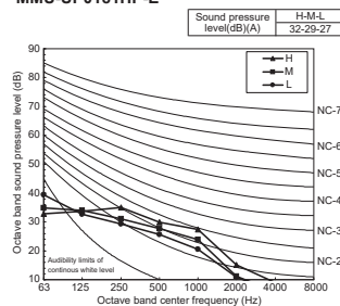
MMU-UP0181HP-E
