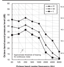
MMU-UP0361H-E
