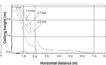
MMU-UP0361, 0481, 0561H-E
