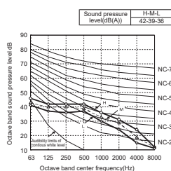
MMU-UP0361WH-E
