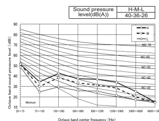
MMU-UP0241SH-E
