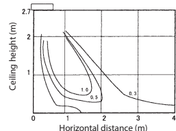
MMU-UP0561WH-E
