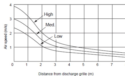
MML-UP0181H-E, MML-UP241H-E
