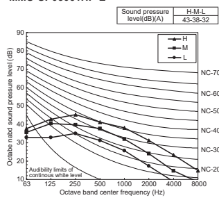
MMU-UP03061HP-E
