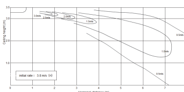
MMC-UP0241, 0271HP-E
