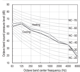
MMY-MUP0801HT8(J)P
