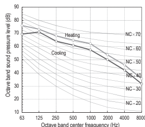
MMY-MUP2201HT8(J)P
