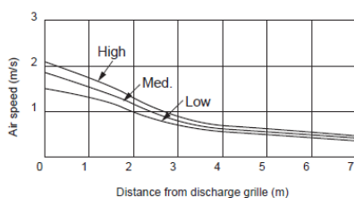
MML-UP0071H-E, MML-UP0091H-E
