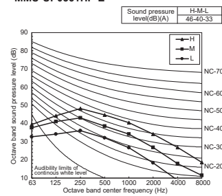
MMU-UP0561HP-E
