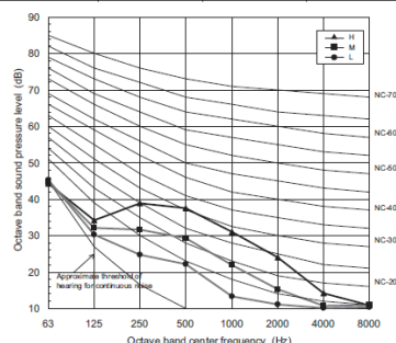
MML-UP0151NH-E
