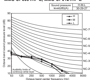
MMU-UP0091HP-E, MMU-UP0121HP-E
