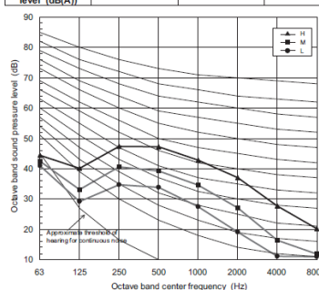
MML-UP0181NH-E
