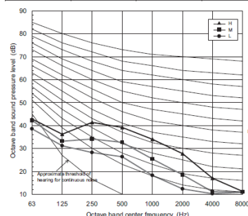
MML-UP0181NH-E
