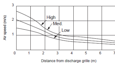
MML-UP0121H-E, MML-UP151H-E
