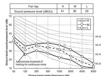
MMC-UP0561HP-E
