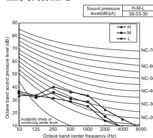
MMU-UP0301HP-E
