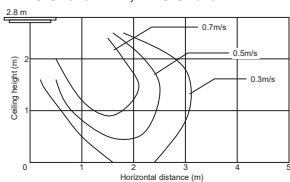
MMU-UP0481HP-E, MMU-UP0561HP-E
