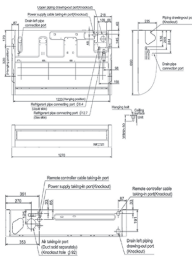
MMC-UP0241HP-E, MMC-UP0271HP-E
