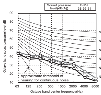
MMU-UP0181SH-E
