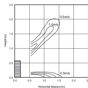
MML-UP0181NH-E
