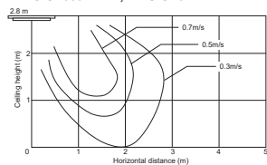
MMU-UP0361HP-E
