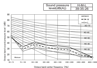
MMU-UP0181SH-E
