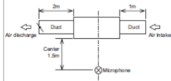
SLIM DUCT &amp; STANDARD DUCT &amp; HIGH STATIC DUCT
