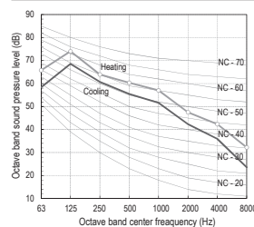
MMY-MUP1201HT8(J)P
